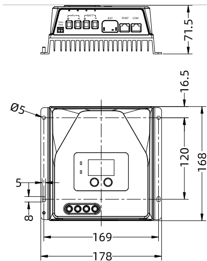
TRC5215
