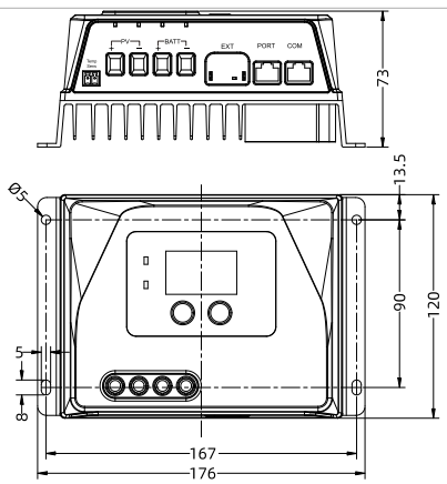
TRC4415/TRC4215
