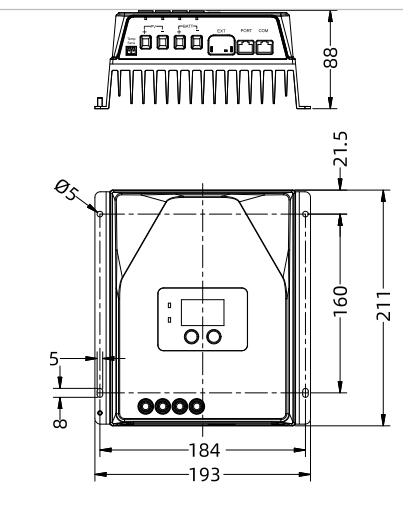
TRC4415/TRC4215
